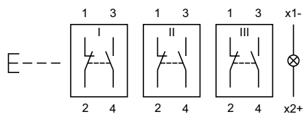
Wiring diagram 25
