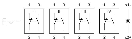
Wiring diagram 28
