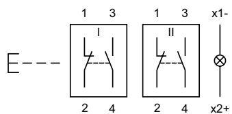
Wiring diagram 23
