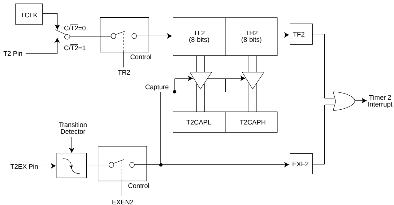
Figure 11. Timer 2 in Capture Mode
