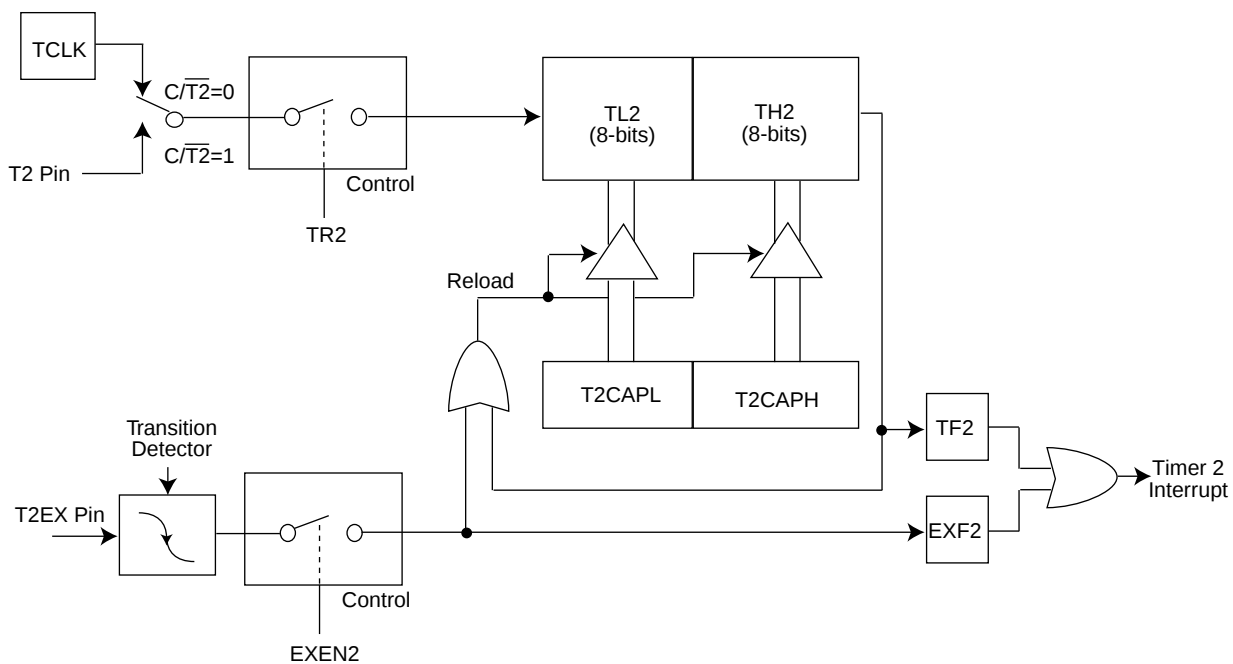
Figure 12. Timer2 in Auto-Reload Mode(DECN=0)
