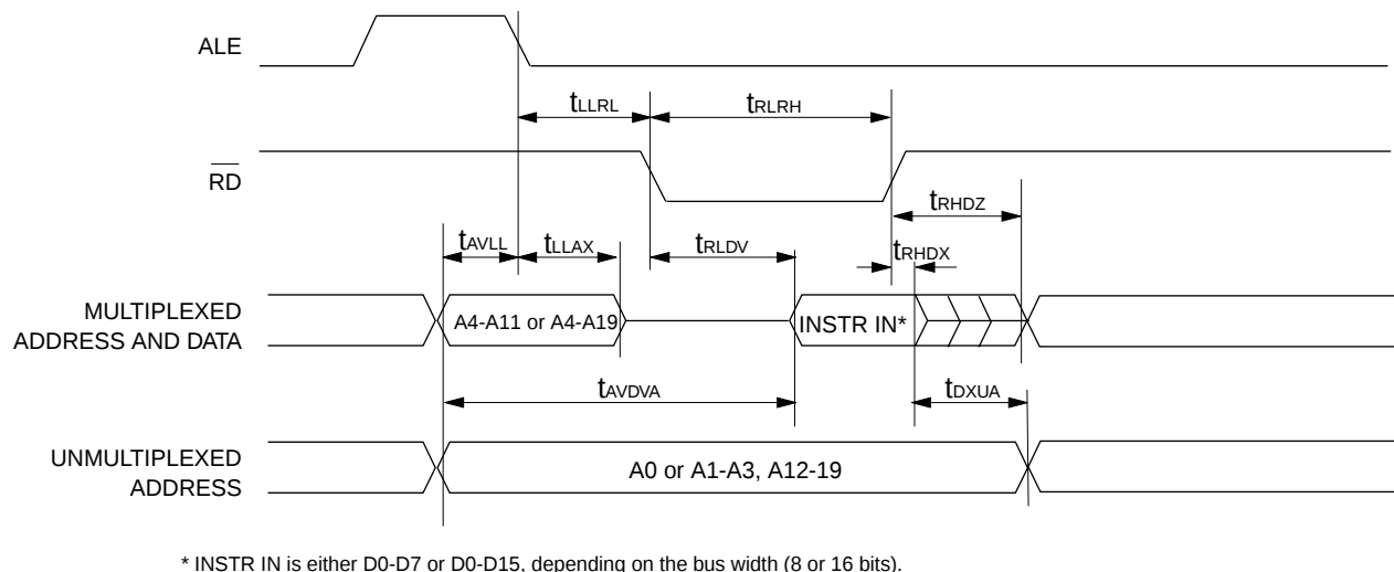
Figure 22. External Data Memory Read Cycle (ALE Cycle)
