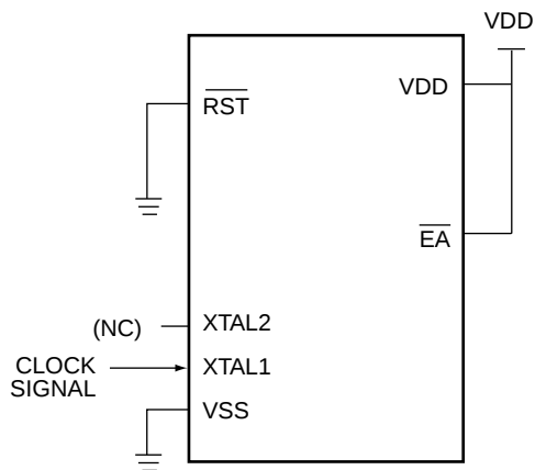
Figure 29. IDD Test Condition, Active Mode All other pins are disconnected
