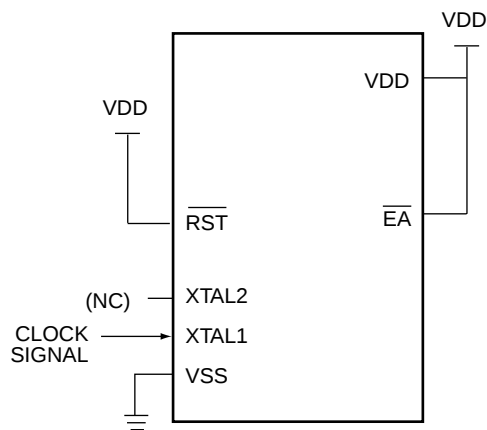
Figure 30. IDD Test Condition, Idle Mode All other pins are disconnected
