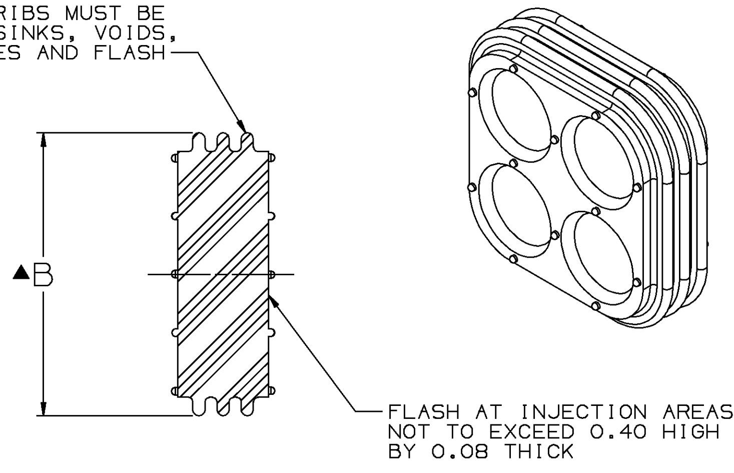
SECTION B-B
