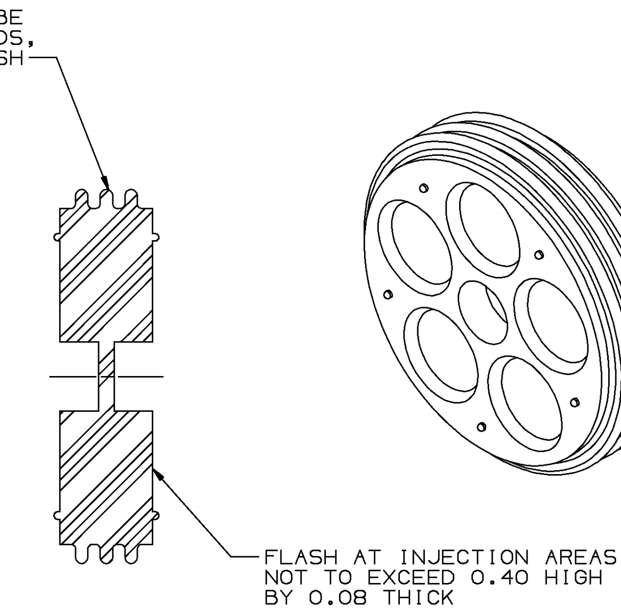
SECTION G-G
