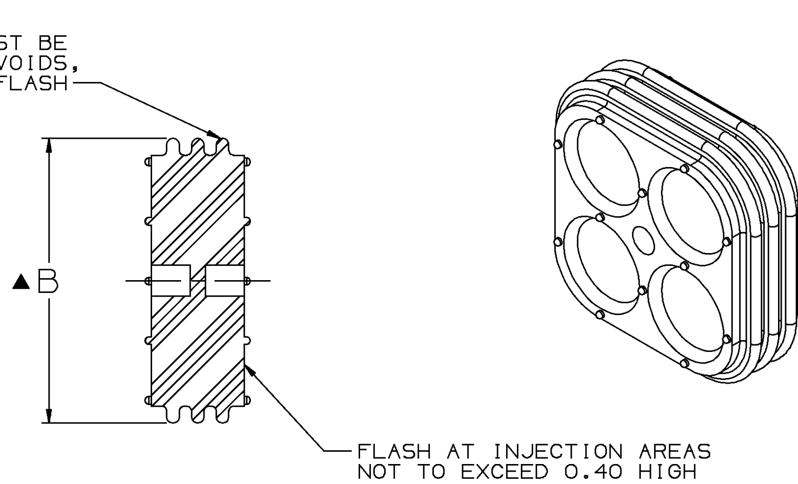
SECTION E-E
