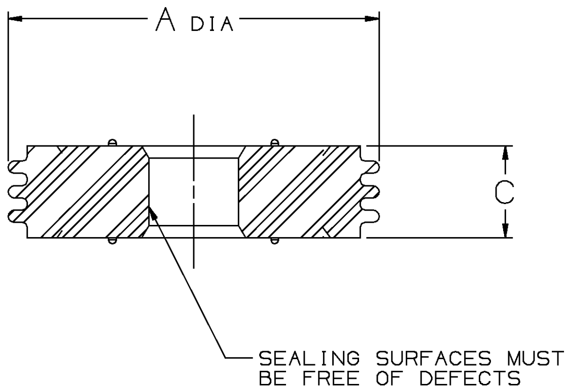
SECTION F-F
