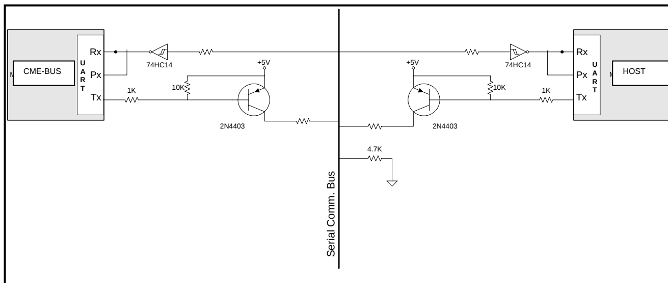
Figure 1. Typical Circuit for Single-line Serial Communication Bus
