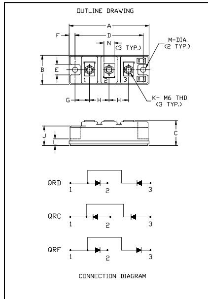
QR_0610T30 Fast Recovery Diode Module
