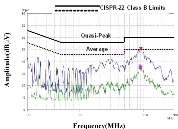
Figure 15. FSD210B Full Range EMI scan(134kHz, with Frequency Modulation) with charger set
