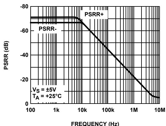
FIGURE 20. PSRR
