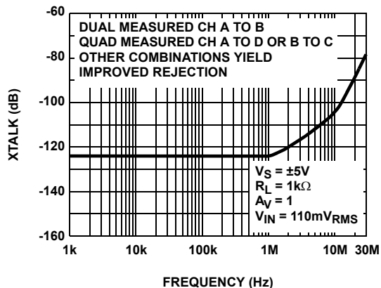
FIGURE 22. CHANNEL SEPARATION
