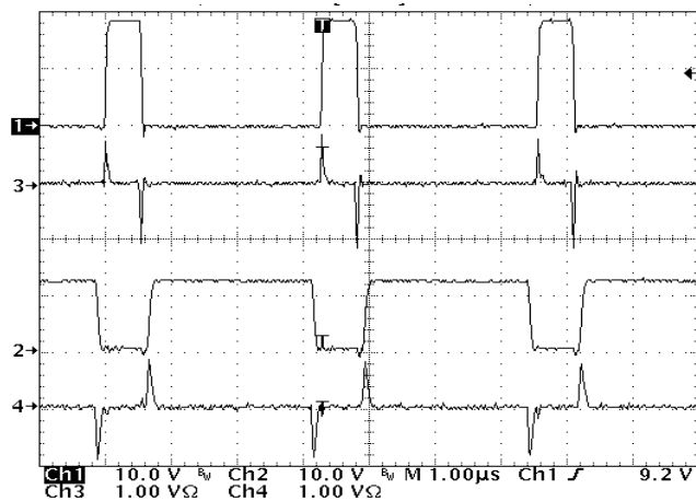
Figure 30 - High side and Low side Drivers peak Current for 1.8V Output Ch1: HDrv2, Ch2: LDrv2, Ch3: High Side Peak Current, Ch4: Low Side Peak Current
