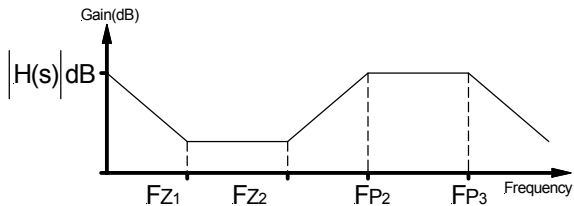
Figure 16- Compensation network with local feedback and its asymptotic gain plot.
