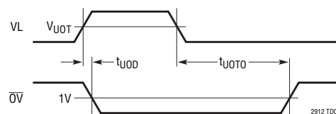
VL Monitor Timing (TMR Pin Strapped to V_{CC} )
