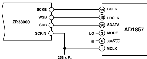
Figure 19. Interface to ZR38000
