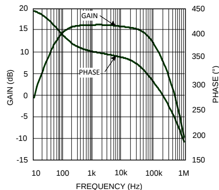
Figure 24. Gain vs. Frequency
