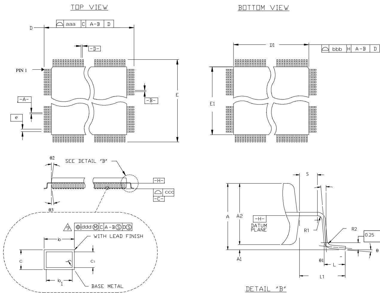
Figure 9-1. 176-lead Thin Quad Flat Pack Package Drawing
