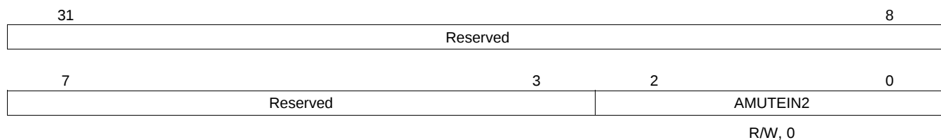
Figure 4-28. CFGMCASP2 Register Bit Layout (0x4000 0020)
