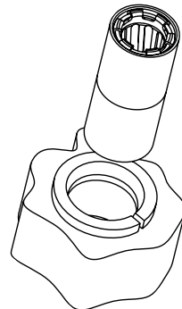
3.6mm RadSert and inner RADSOK®
