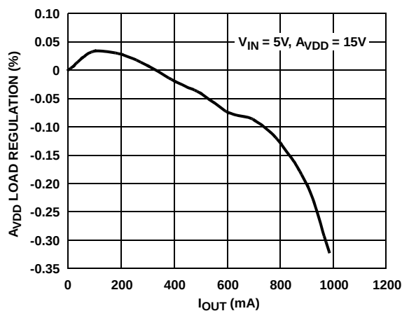
FIGURE 2. A_{VDD} LOAD REGULATION vs I_{OUT}
