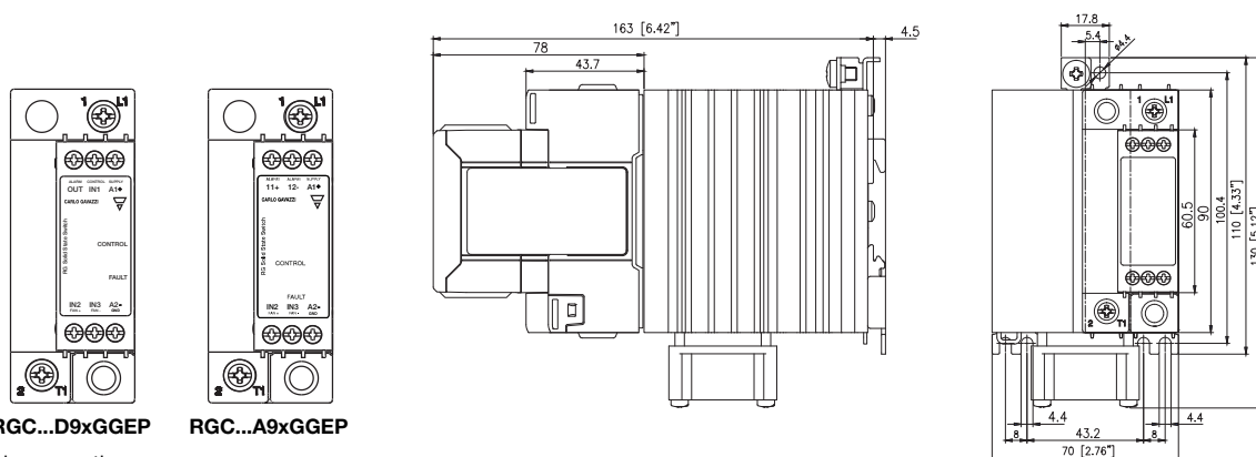
RGC...90GGEP, RGC...92GGEP
