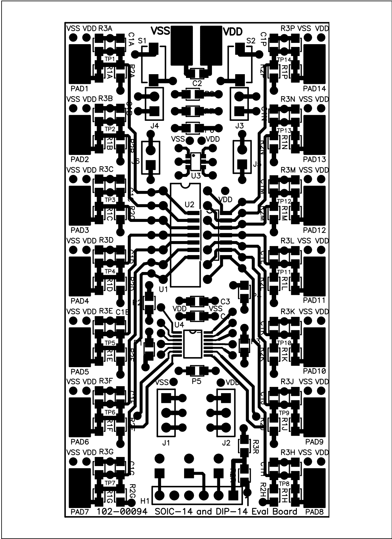
FIGURE A-5: Board Layout – Top Layer + Silk-Screen.
