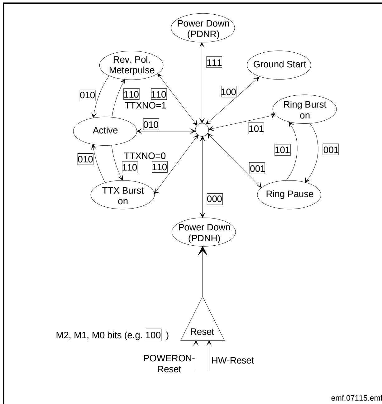
Figure 31 Operating Modes
