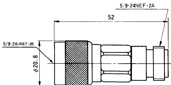
AT-400 Type
