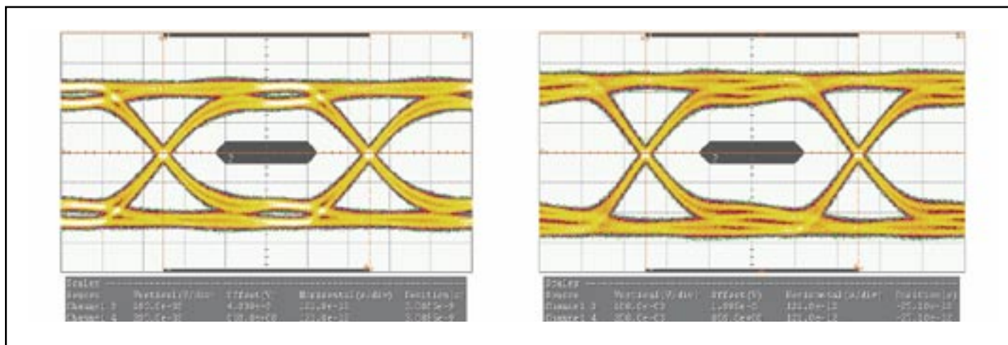
Figure 4. TP3 (Rx) - "Switch at receiver side" with 2-meter cable eye-measurements (left is with switch, right is without switch), refer to figure 2 for the test set up.
