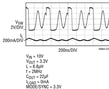
Fixed Frequency No Load Waveform
