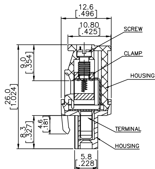
SECTION P-P
