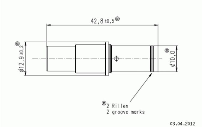
Drawing Dimensions in mm (Inch)
