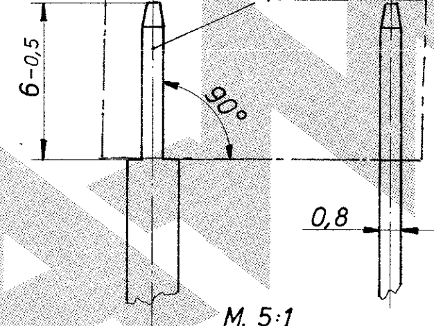
DETAIL "Y"
