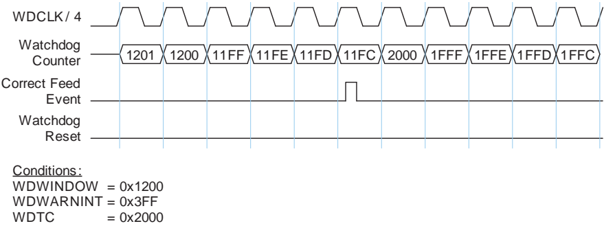
Fig 61. Correct Watchdog Feed with Windowed Mode Enabled
