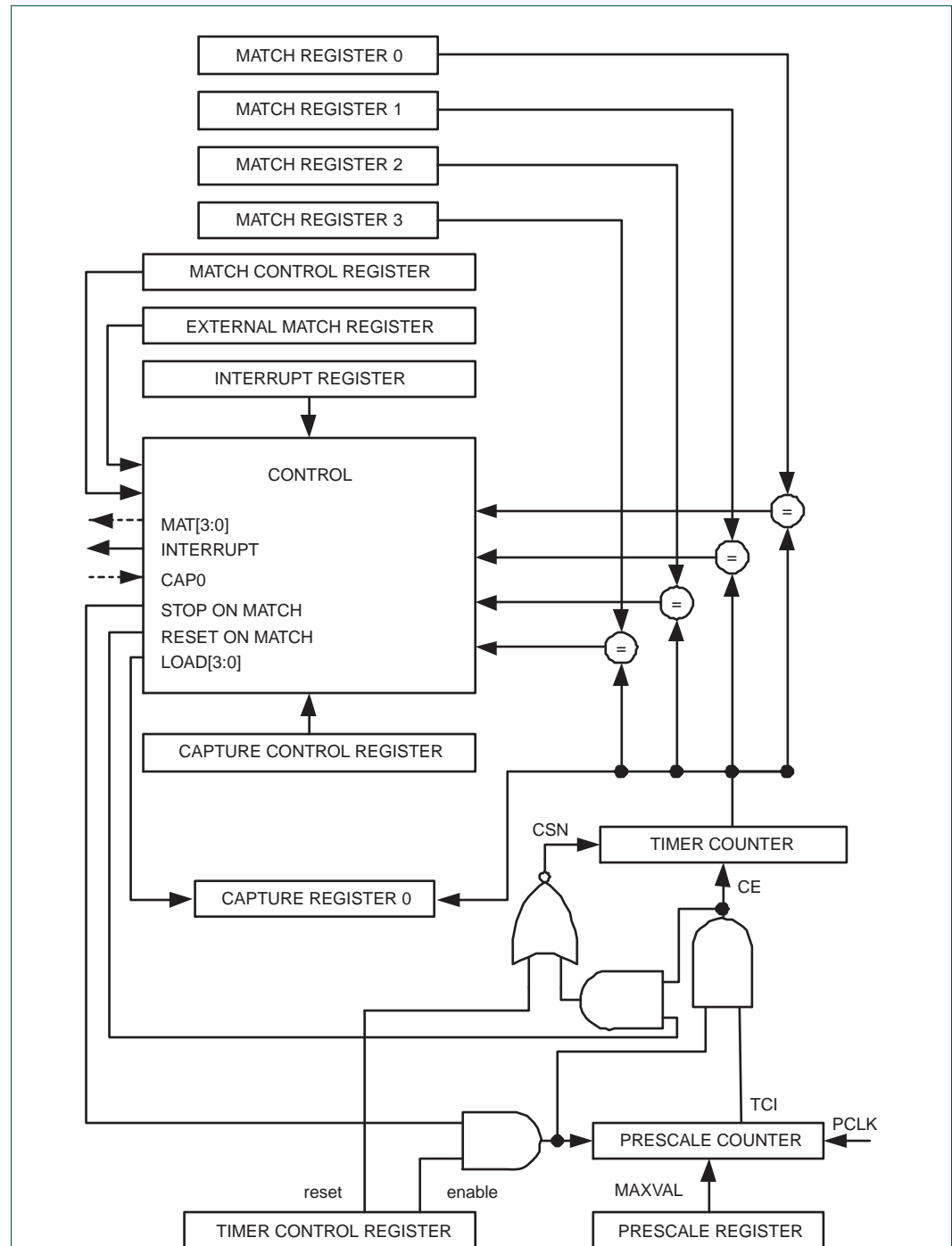
Fig 56. 32-bit counter/timer block diagram
