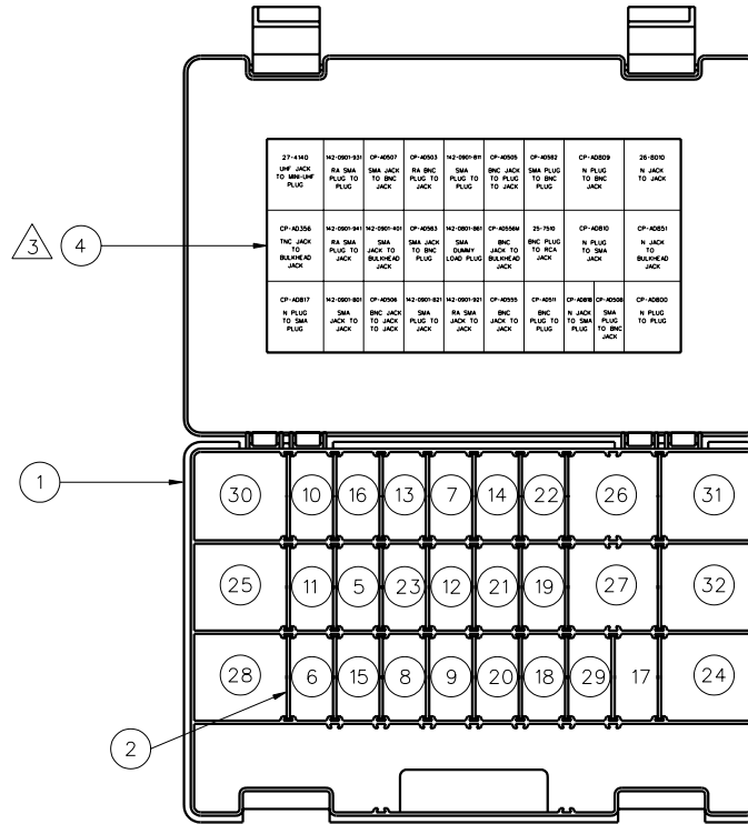
OPEN VIEW
