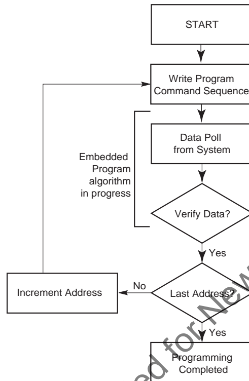
Figure 9.2 Program Operation
