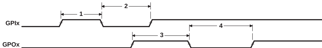
Figure 8-80. GPIO Port Timing
