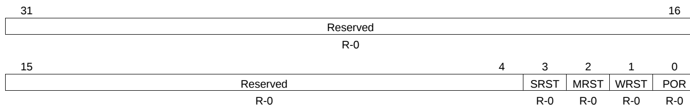
Figure 8-7. Reset Type Status Register (RSTYPE) [Hex Address: 029A 00E4]
