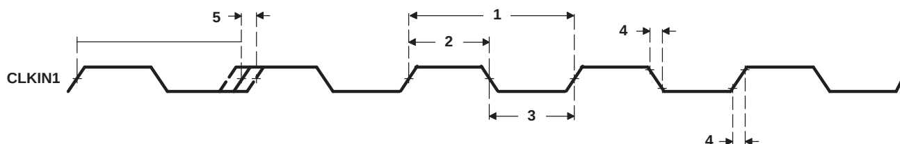
Figure 8-21. CLKIN1 Timing
