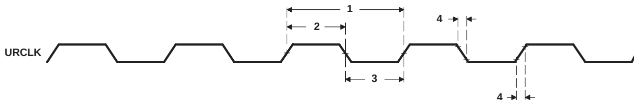
Figure 8-75. URCLK Timing
