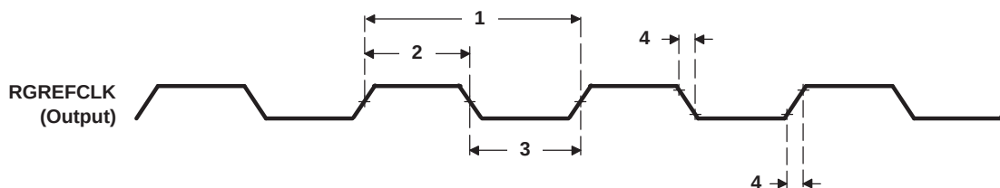
Figure 8-68. RREFCLK Timing
