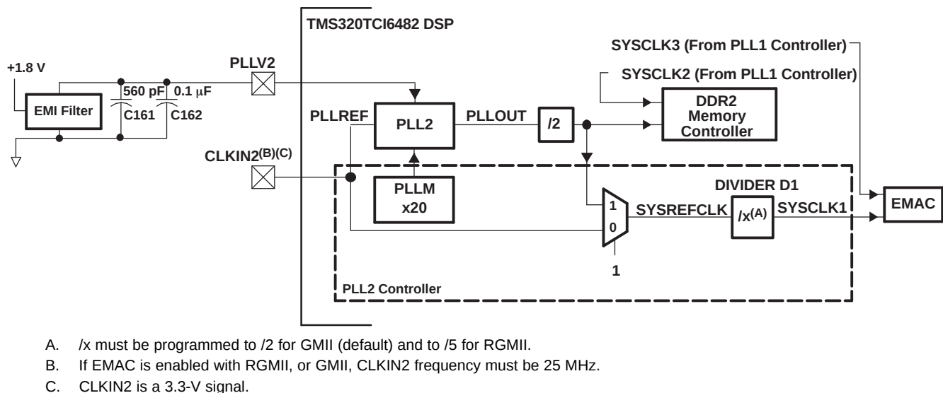
Figure 8-23. PLL2 Block Diagram
