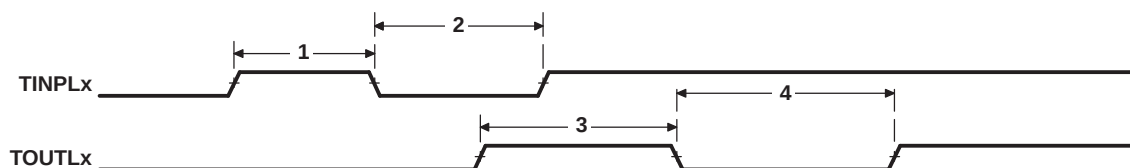
Figure 8-73. Timer Timing
