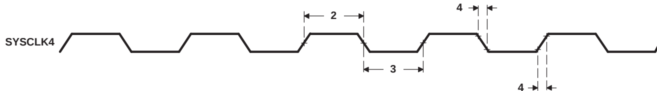
Figure 8-22. SYSCLK4 Timing
