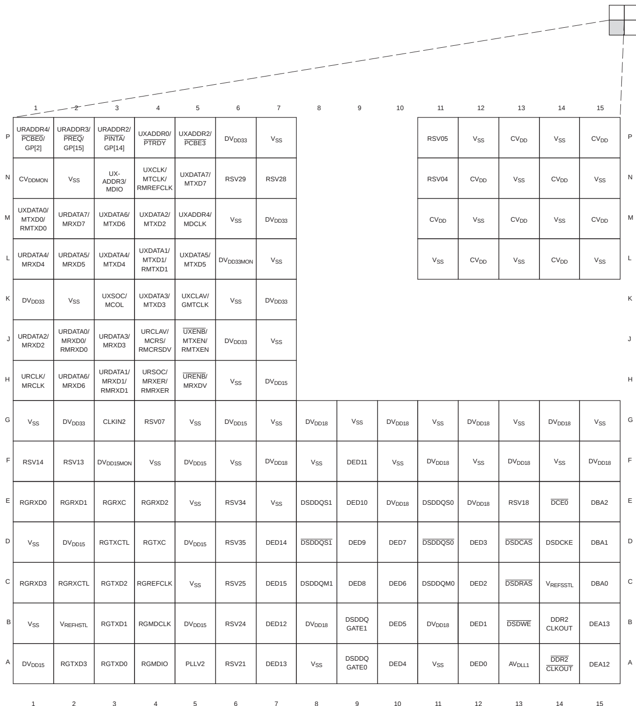
Figure 2-5. TCI6482 Pin Map (Bottom View) [Quadrant D]
