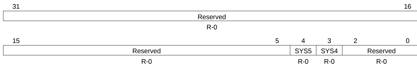
Figure 8-19. PLLDIV Divider Ratio Change Status Register (DCHANGE) [Hex Address: 029A 0144]
