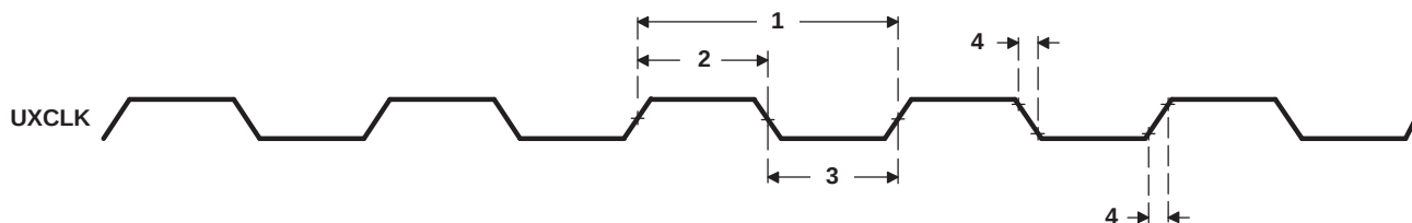
Figure 8-74. UXCLK Timing
