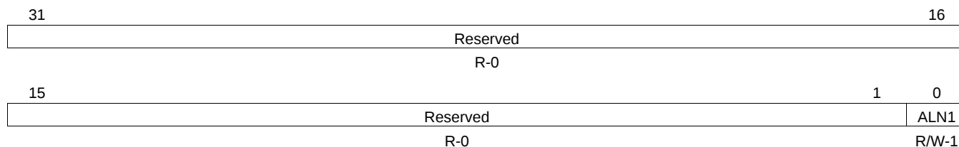
Figure 8-27. PLL Controller Clock Align Control Register (ALNCTL) [Hex Address: 029C 0140]
