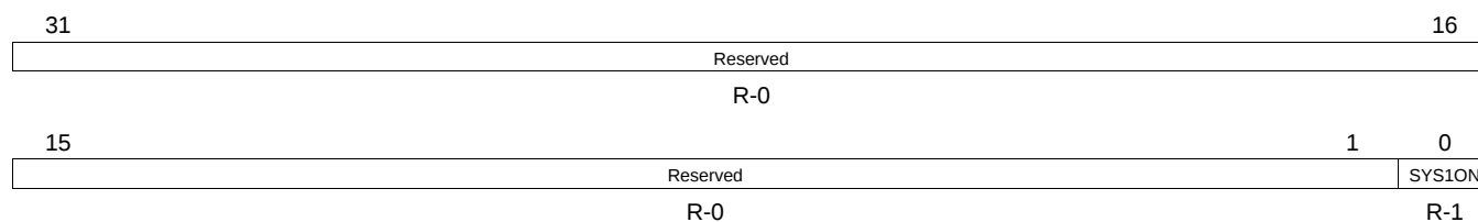
Figure 8-29. SYSCLK Status Register [Hex Address: 029C 0150]
