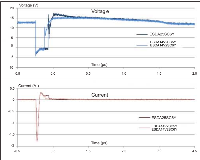
Figure 9. ISO7637-2 pulse 3a response ( V_S = -150\text{ V} )
