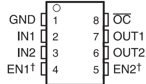
TPS2090, TPS2091, AND TPS2092 D PACKAGE
