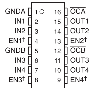
TPS2095, TPS2096 AND TPS2097 D PACKAGE
