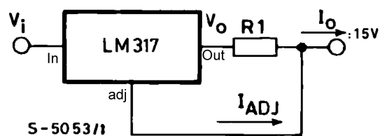
Figure 10. Current regulator
