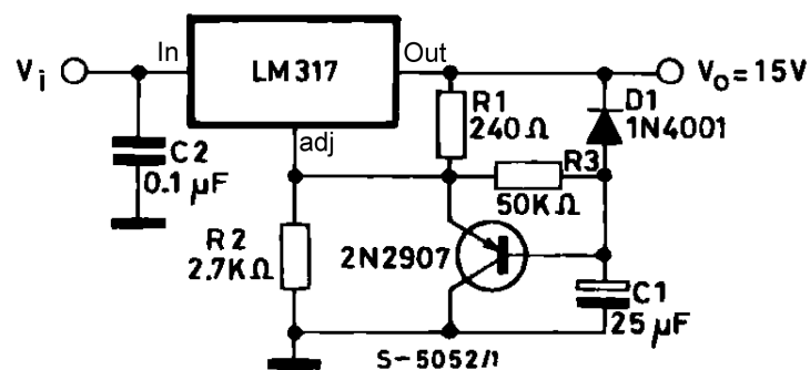
Figure 9. Slow turn-on 15 V regulator
