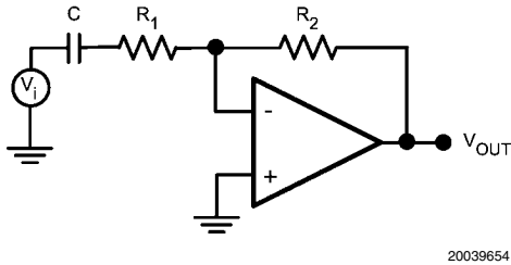
FIGURE 5. Highpass Filter
