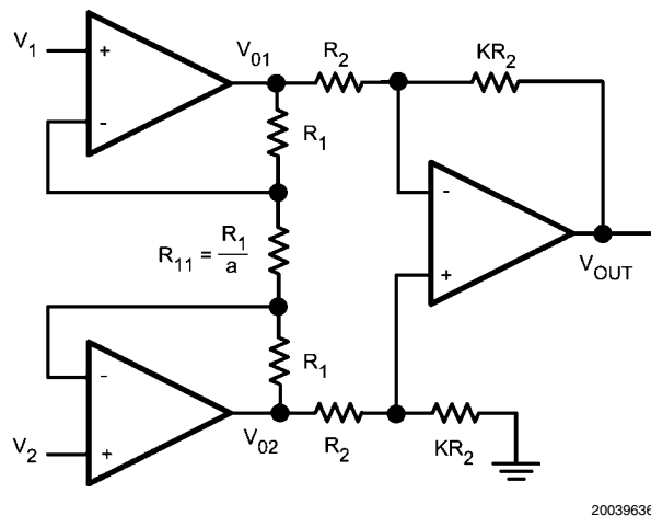
FIGURE 1. Instrumentation Amplifier
