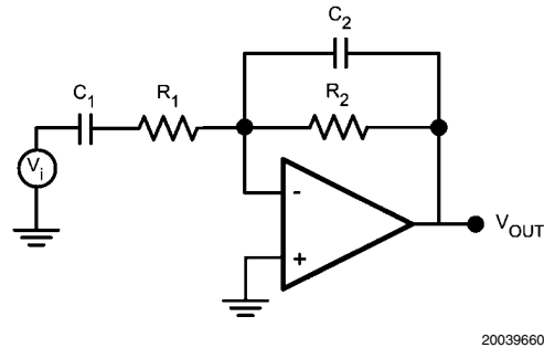
FIGURE 7. Bandpass Filter
