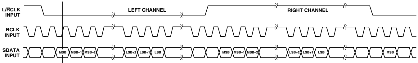
Figure 2. I²S-Justified Mode
