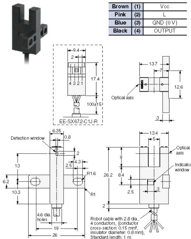
Terminal Arrangement
