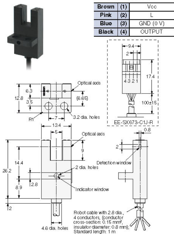
Terminal Arrangement
