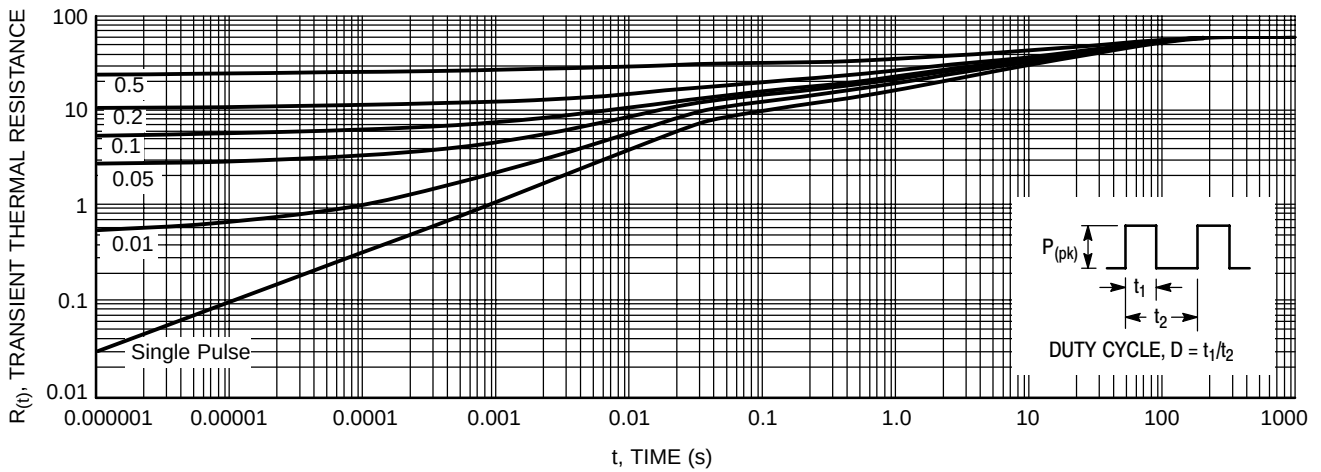
Figure 8. Thermal Response
