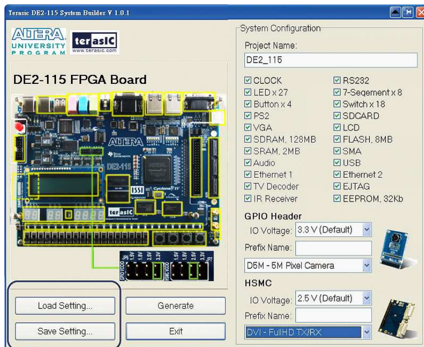
Figure 5-7 Project Settings
