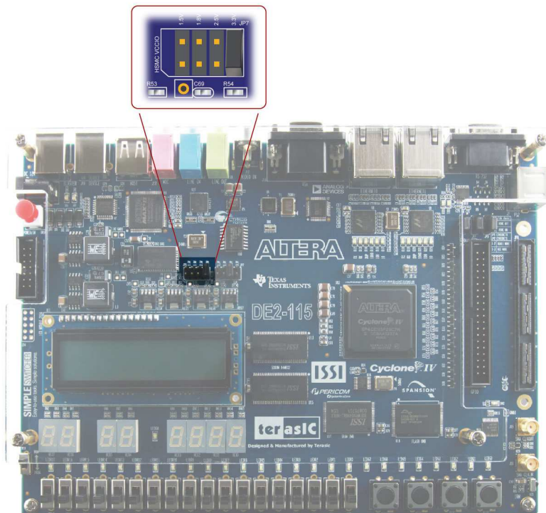
Figure 4-17 GPIO VCCIO supply voltage setting header
