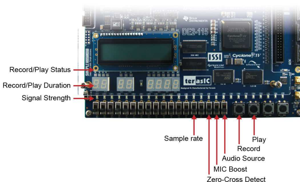
Figure 6-25 Man-Machine Interface of Audio Recorder and Player
