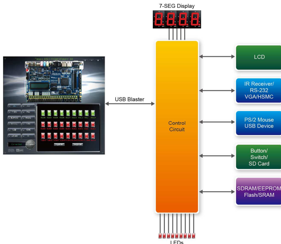
Figure 3-2 The DE2-115 Control Panel concept
