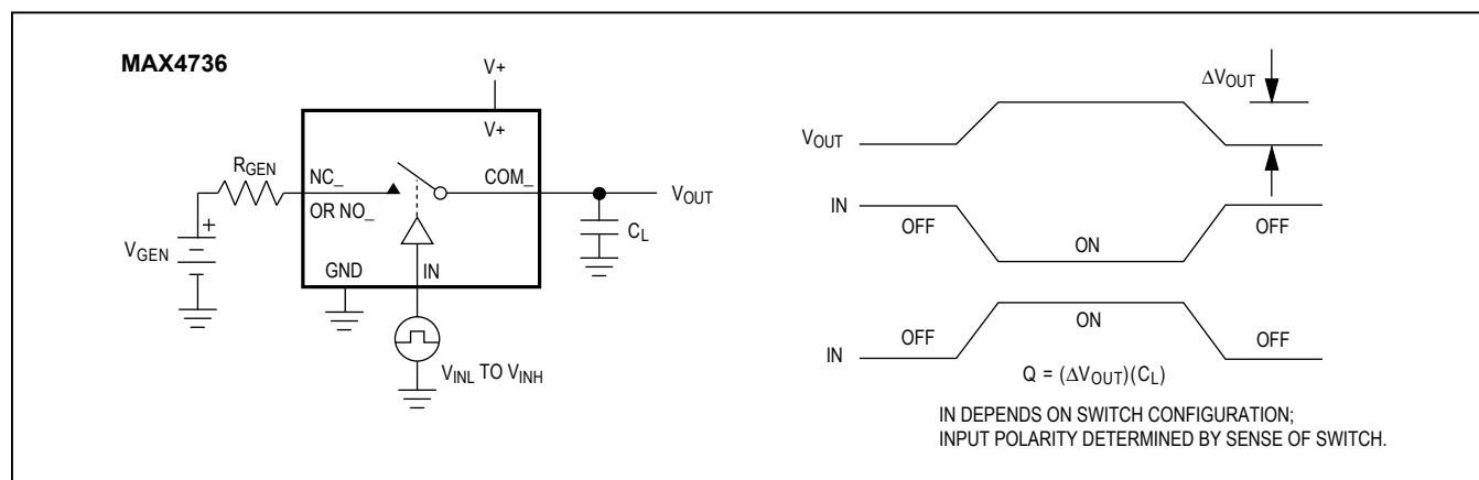
Figure 3. Charge Injection
