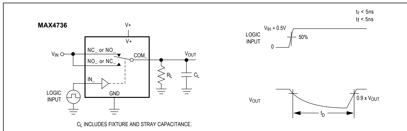
Figure 2. Break-Before-Make Interval
