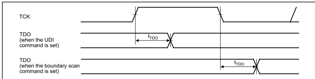
Figure 23.3 UDI Data Transfer Timing
