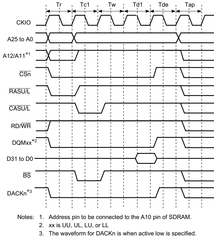
Figure 7.17 Basic Timing for Single Read (Auto Precharge)
