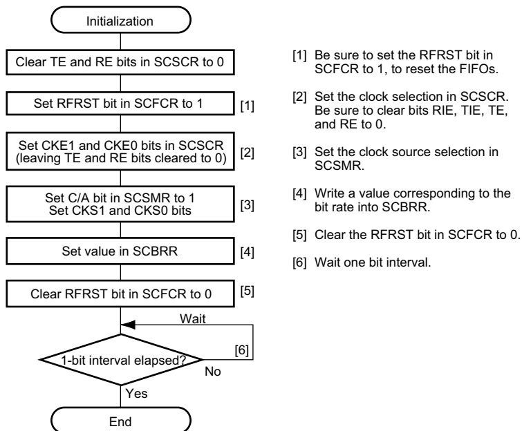
Figure 16.13 Sample SCIF Initialization Flowchart (2) (Reception)
