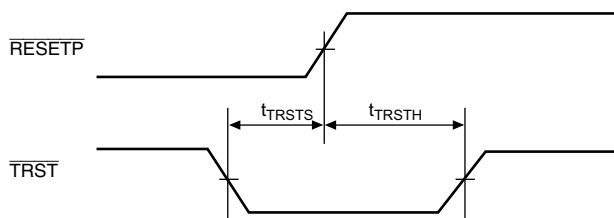
Figure 25.55 \overline{\text{TRST}} Input Timing (Reset Hold)
