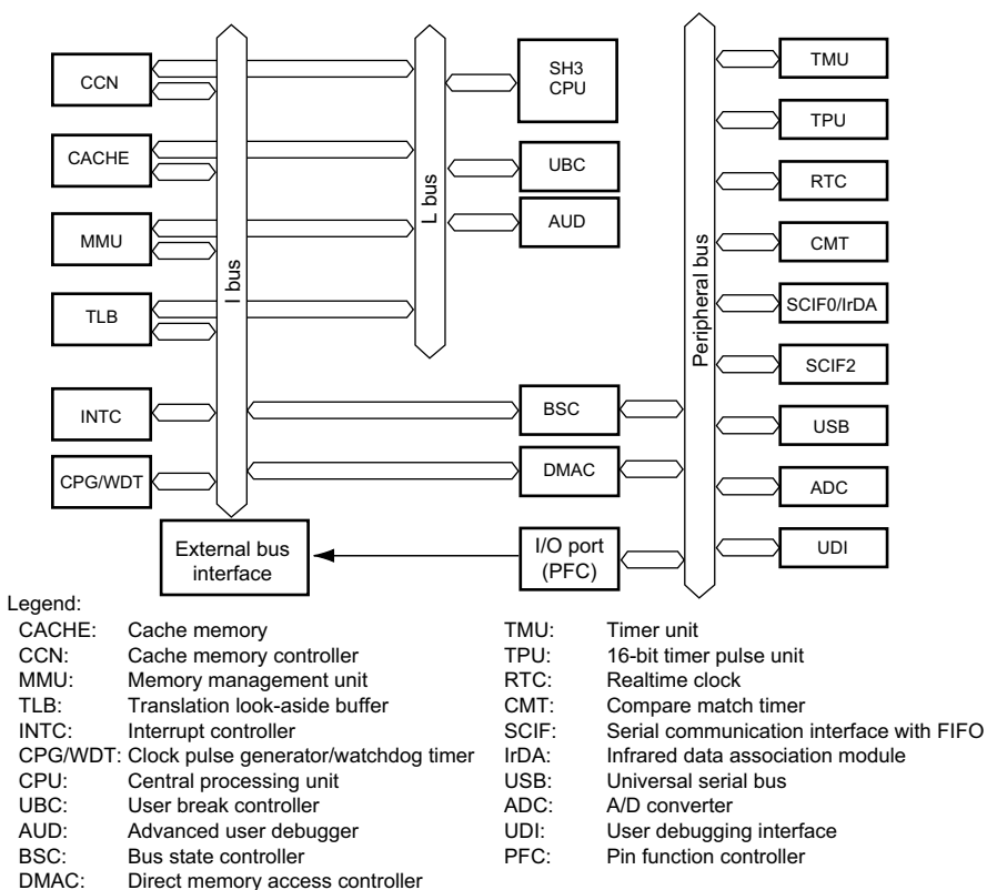
Figure 1.1 Block Diagram of SH7705
