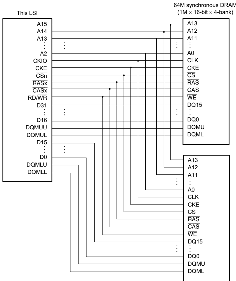
Figure 7.14 Example of 64-MBit Synchronous DRAM Connection (32-Bit Data Bus)
