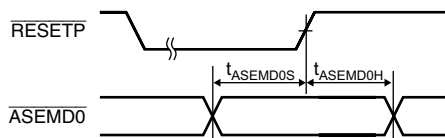
Figure 25.57 \overline{\text{ASEMD0}} Input Timing
