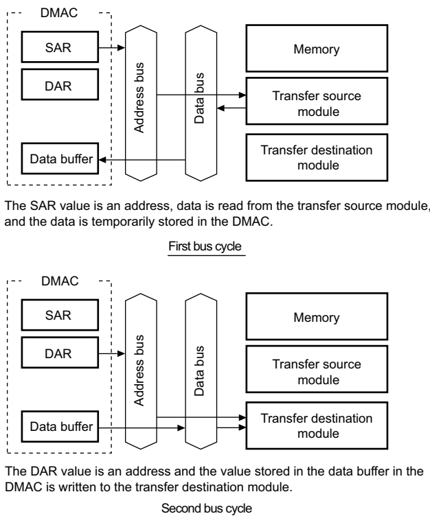
Figure 8.5 Data Flow of Dual Address Mode
