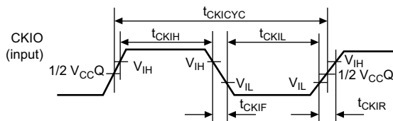
Figure 25.3 CKIO Clock Input Timing
