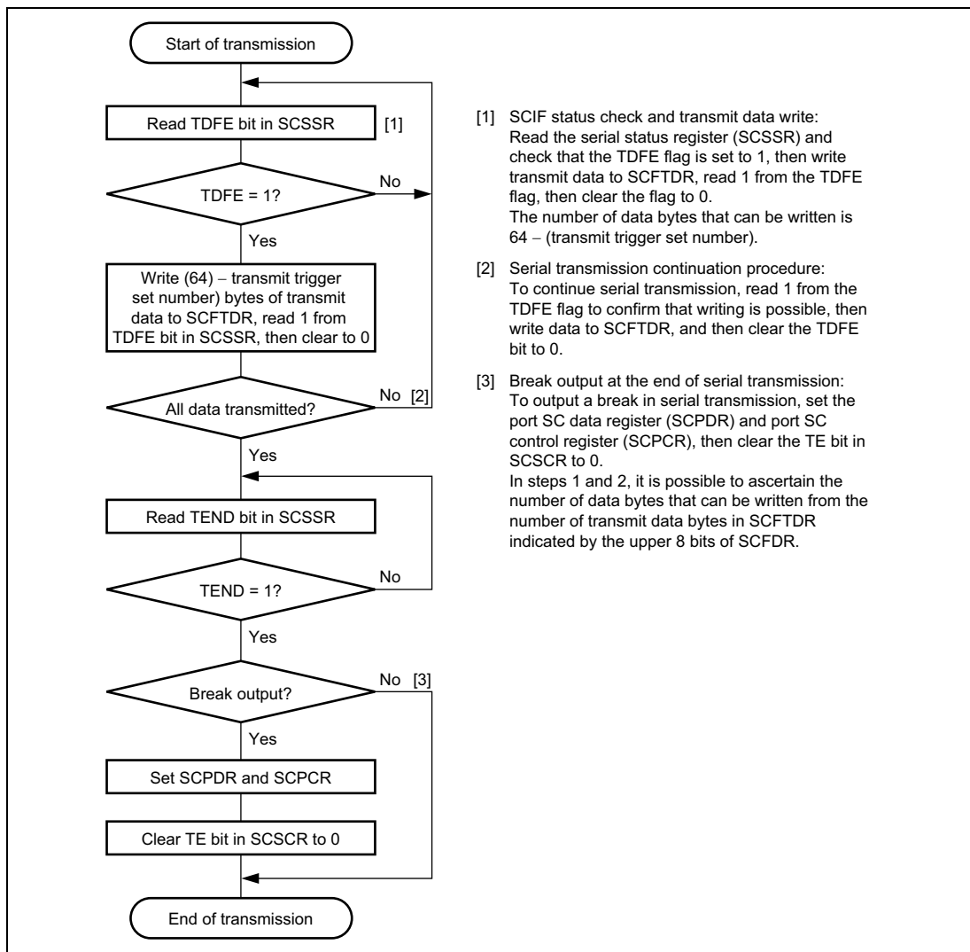
Figure 16.3 Sample Serial Transmission Flowchart
