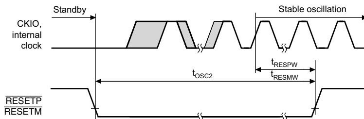
Figure 25.6 Oscillation Settling Time at Standby Return (Return by Reset)
