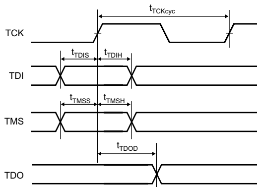
Figure 25.56 UDI Data Transfer Timing
