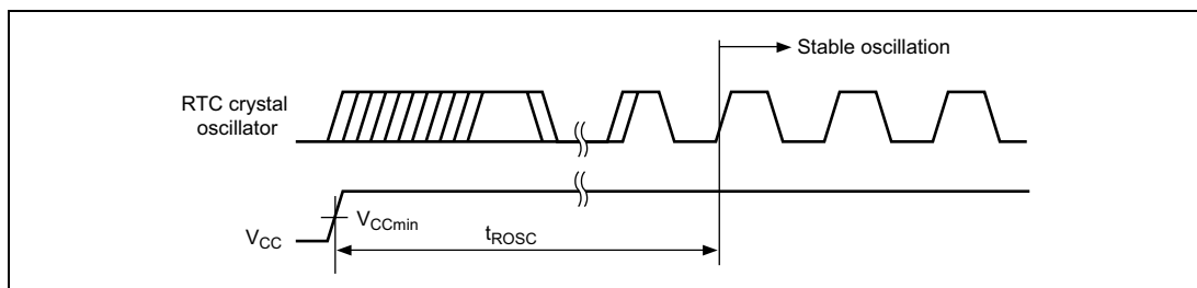
Figure 25.47 Oscillation Settling Time when RTC Crystal Oscillator Is Turned On
