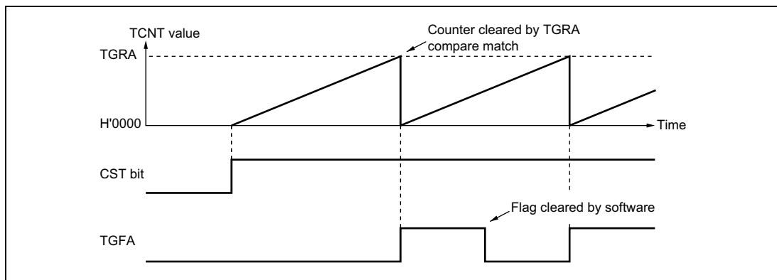
Figure 14.4 Periodic Counter Operation
