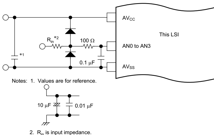
Figure 21.6 Example of Analog Input Protection Circuit
