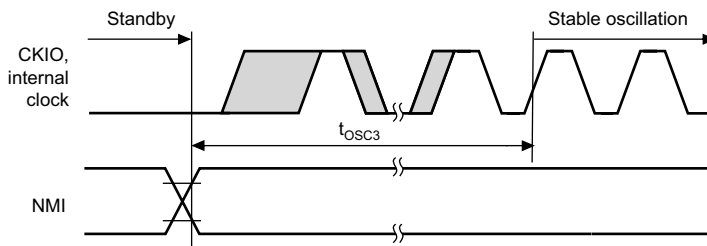
Figure 25.7 Oscillation Settling Time at Standby Return (Return by NMI)
