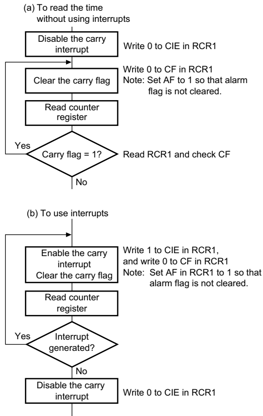
Figure 15.3 Reading the Time
