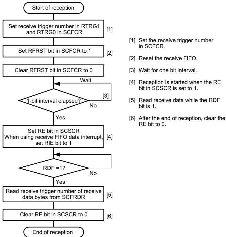
Figure 16.15 Sample Serial Reception Flowchart (2) (Second and Subsequent Reception)
