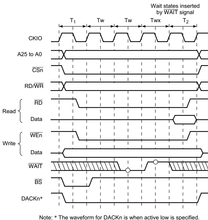
Figure 7.9 Wait State Timing for Normal Space Access (Wait State Insertion by \overline{\text{WAIT}} Signal)
