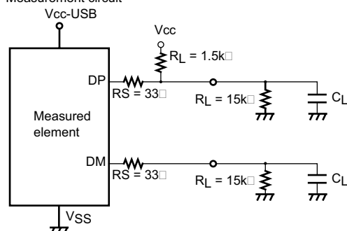
Measurement circuit
