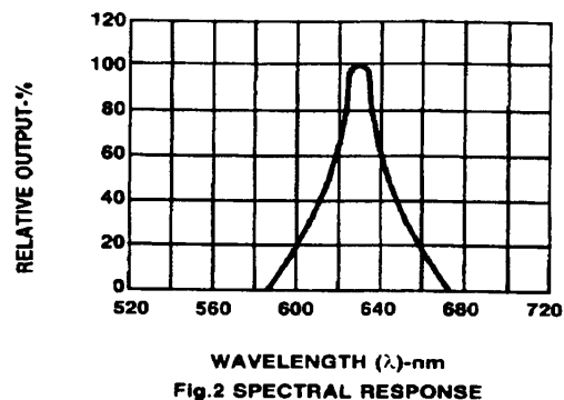
Fig.2 SPECTRAL RESPONSE
