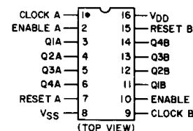
CD4518B, CD4520B TERMINAL ASSIGNMENT
