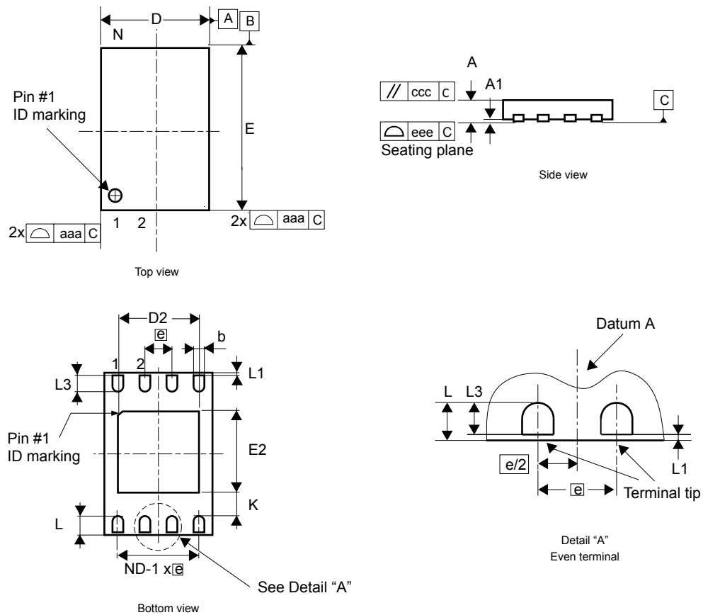
Figure 24. UFDFPN8 - Outline
