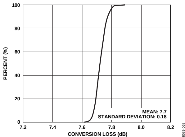
Figure 23. Conversion Loss Distribution
