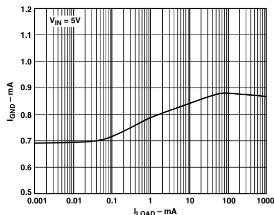
TPC 6. I_{GND} vs. I_{LOAD} ( V_{IN} = 5 V)
