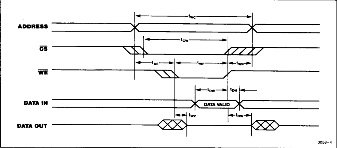
Write Cycle
