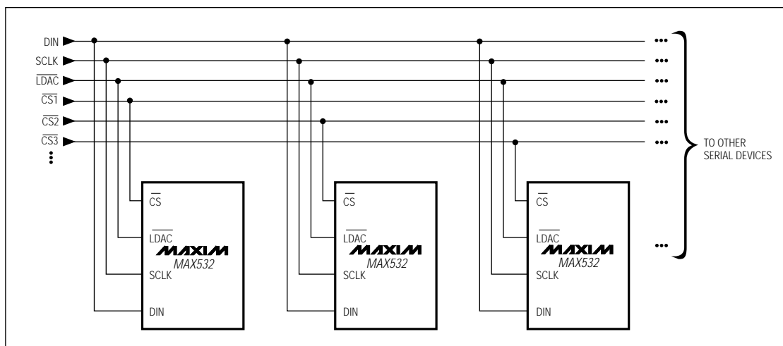
Figure 7. Multiple devices sharing a common DIN line may be simultaneously updated by bringing \overline{LDAC} low. \overline{CS1} , \overline{CS2} , \overline{CS3} , . . . , are driven separately, thus controlling which data are written to devices 1, 2, 3, . . . .
