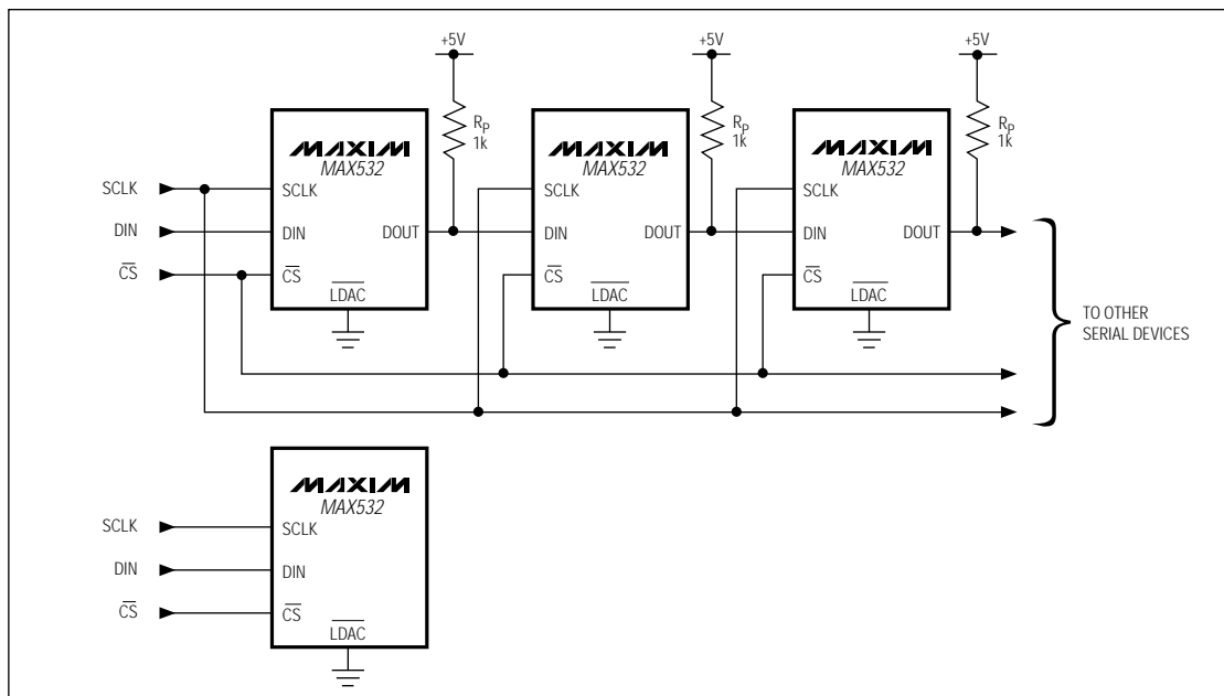
Figure 6. Daisy-chained or individual MAX532s are simultaneously updated by bringing \overline{CS} high when using the 3-wire interface ( \overline{LDAC} = \text{DGND} ).
