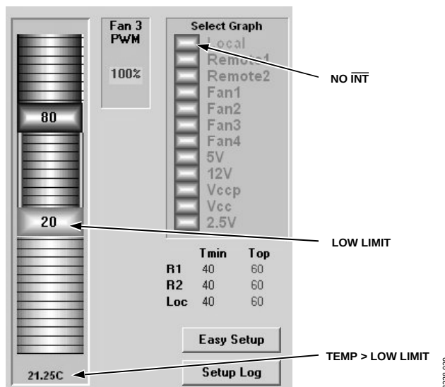
Figure 29. Temperature > Low Limit: No INT
