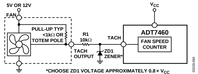
Figure 50. Fan with Strong TACH Pull-Up to > V_{CC} or Totem-Pole Output, Clamped with Zener and Resistor
