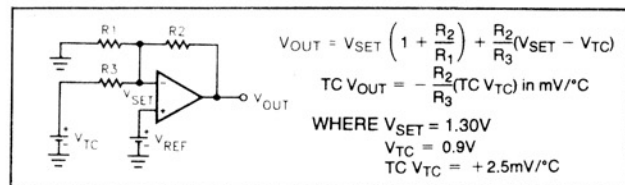
Figure 5. Maxim's Generation of Negative Temperature Coefficients.
