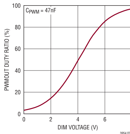
Figure 4. PWMOUT Duty Ratio vs DIM Voltage for R_{DIM} = 124k
