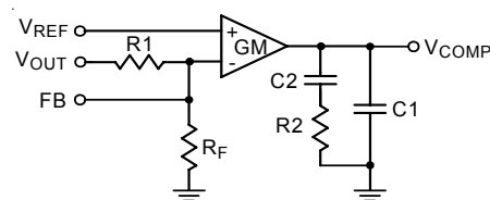
Figure 12. Type II Compensator
