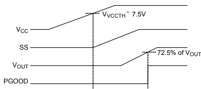
Figure 1. Power on Sequence
