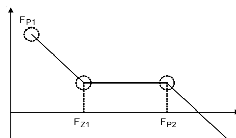
Figure 13. Gain Curve of Type II Compensator
