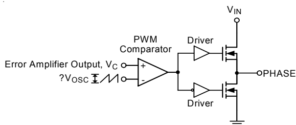
Figure 10. PWM Modulator
