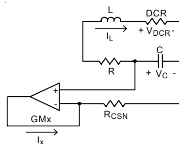
Figure 3. DCR Current Sense Circuit
