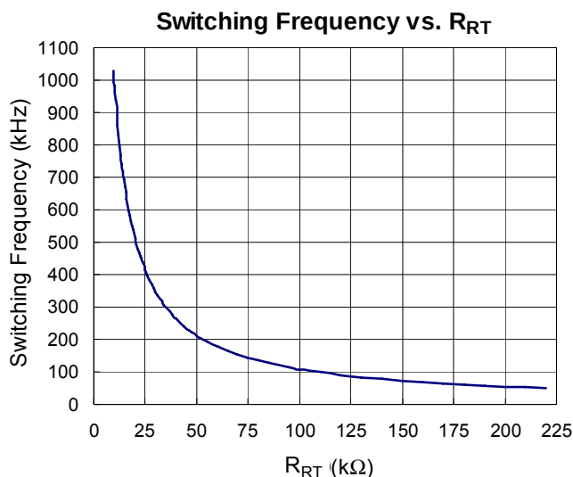
Figure 2. Switching Frequency vs. RT Resistance
