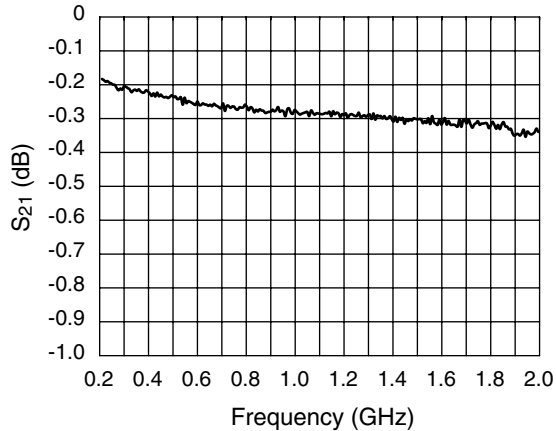
Insertion Loss
